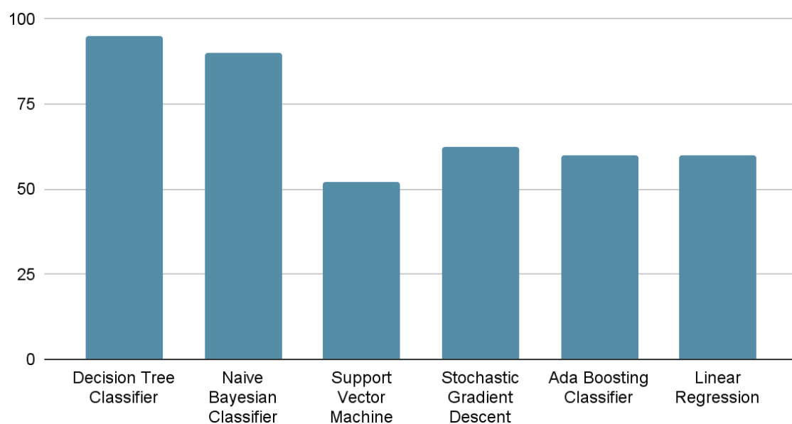
Figure 5: Comparison of accuracies of the machine learning models.
