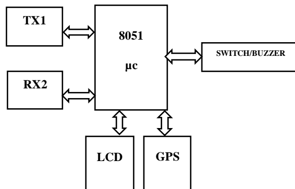
Figure 2.1.1: Module in Ambulance/Emergency Service vehicle
