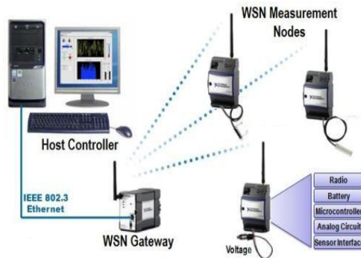
Figure 2.2.1: Data Is Transmitted From All Locations To The Main System
