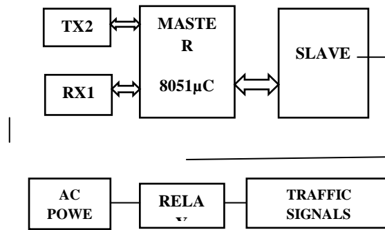
Figure 2.1.2: Module At Traffic Signal Post
