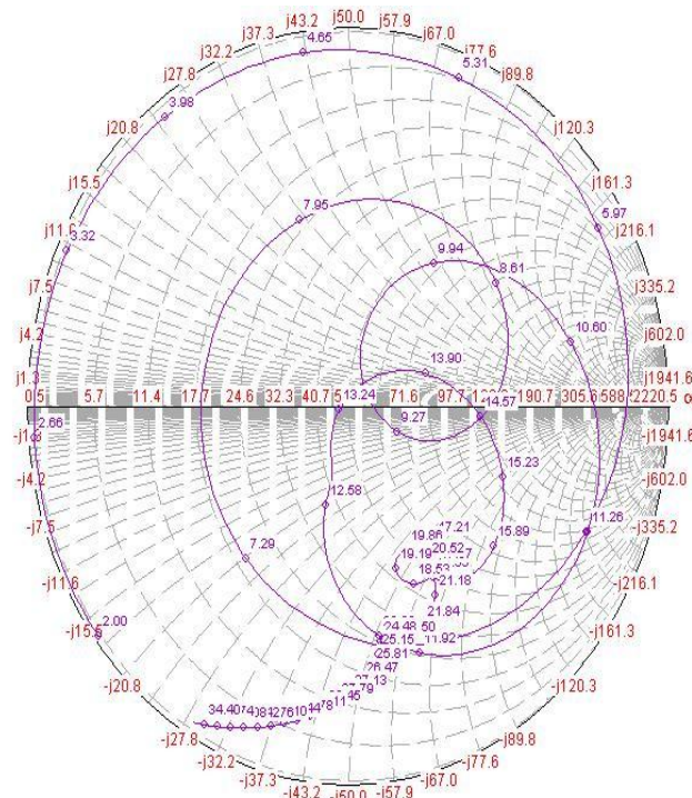
Figure11: Simulated Smith Chart for slotted antenna
