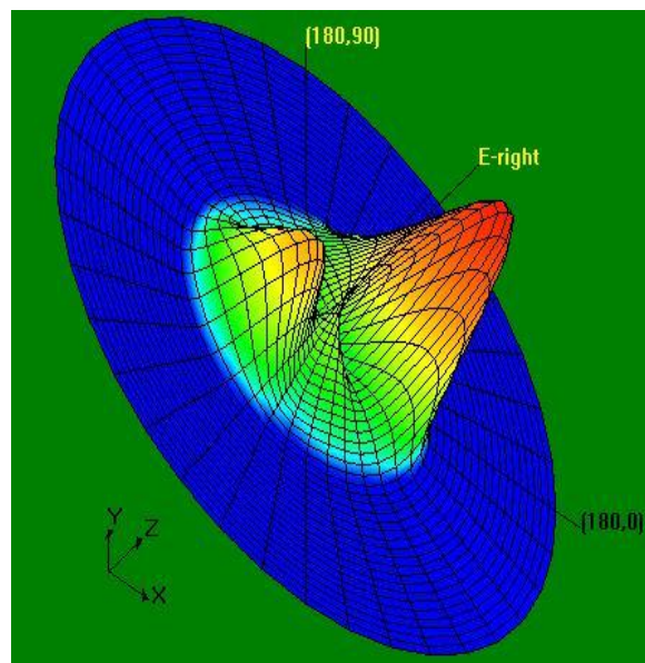
Figure 9: E-Plane Radiation Pattern (3D) for slotted antenna at 13.30 GHz
