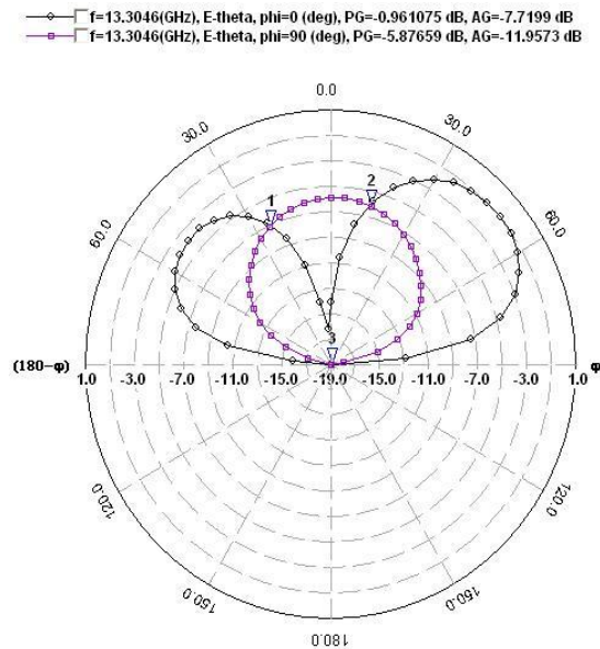
Figure7: E-Plane Radiation Pattern for slotted antenna at 13.30 GHz
