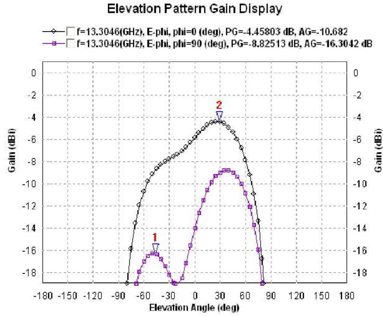
Figure 14: H-Plane Radiation Pattern (2D) for slotted antenna at 13.30GHz
