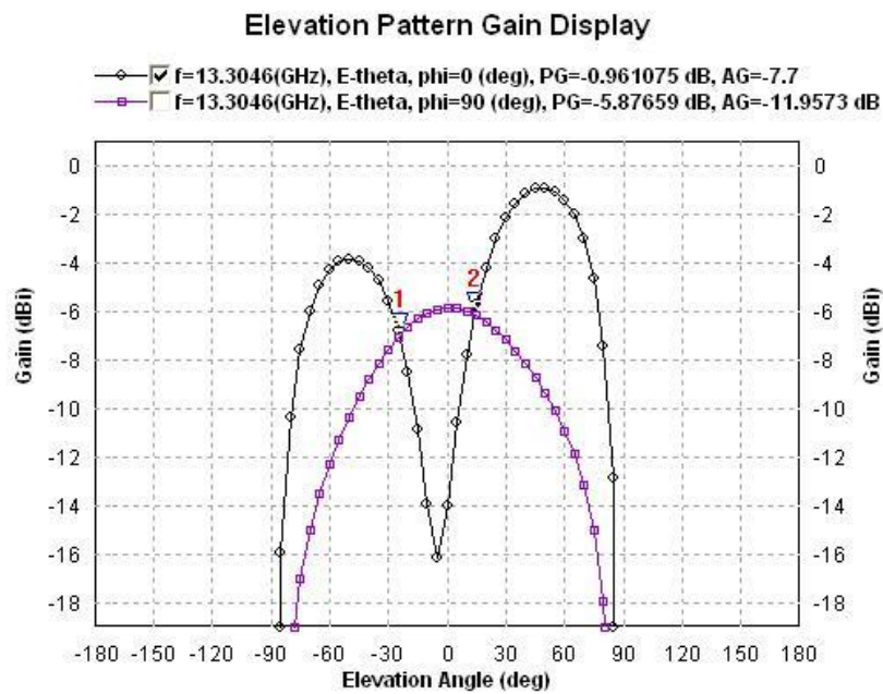
Figure 13: E-Plane Radiation Pattern (2D) for slotted antenna at 13.30 GHz
