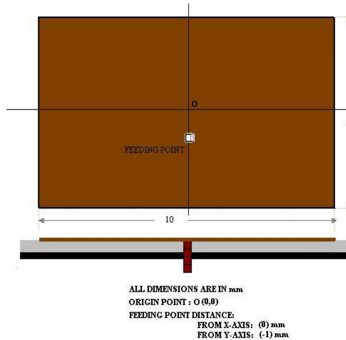
Figure 1. Conventional Antenna configuration
