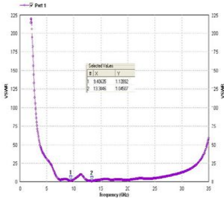
Figure 12: Simulated VSWR for slotted antenna
