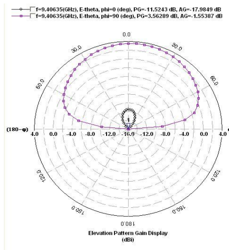
Figure 5: E-Plane Radiation Pattern for Slotted Antenna at 9.40 GHz
