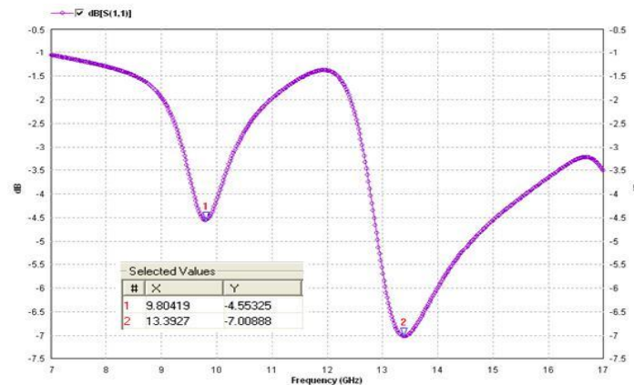
Figure 3: Return Loss vs. Frequency (Conventional Antenna)
