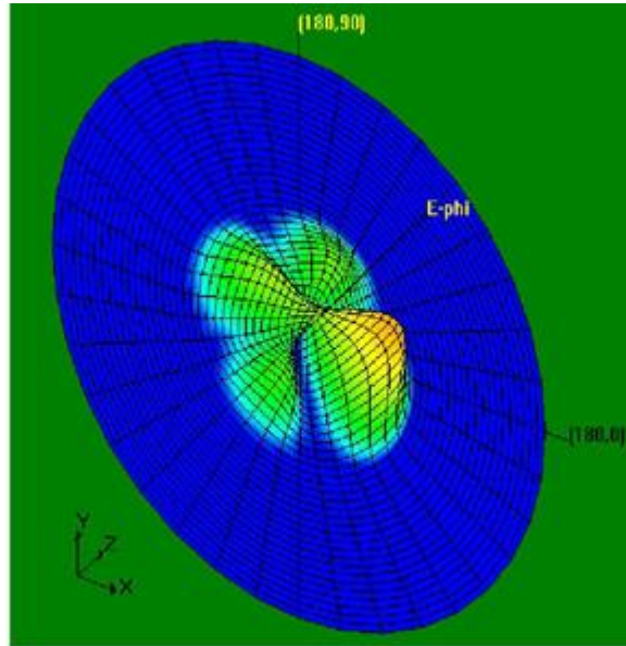
Figure 10: H-Plane Radiation Pattern (3D) for slotted antenna at 13.30 GHz
