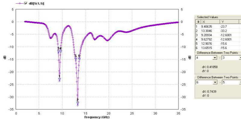
Figure 4: Return Loss vs. Frequency (Slotted Antenna)
