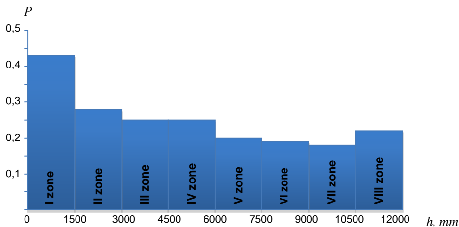
Figure 3: The dependence of the probability of occurrence of unacceptable deviations on shell height.
