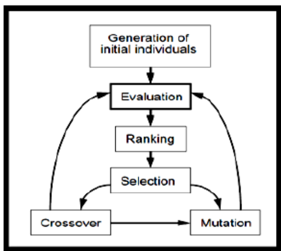
Figure 5: The basic structure of a GA.
