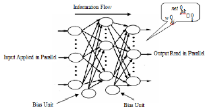
Figure 6: A simple Bp neural network.
