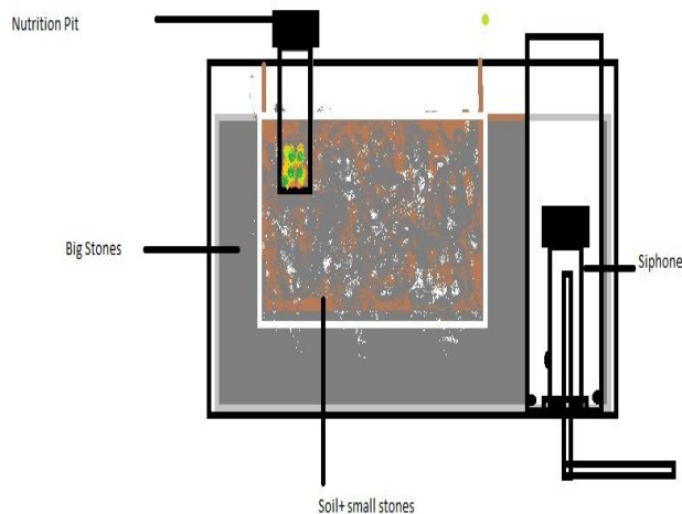
Figure 3: Design of Grow Bed.
