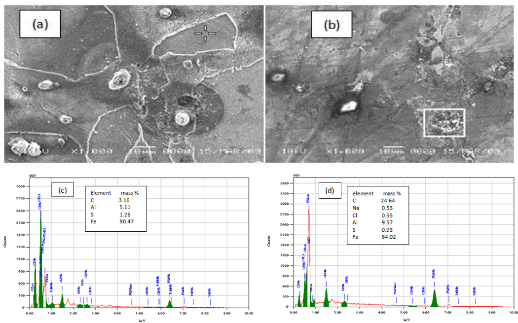
Figure 4: SEM micrographs of as cast of Fe-1.24Al-0.55C alloy after corroded (a). SE image in 0.05M H 2 SO 4 0.05M (b). SE image in 0.5% NaCl. EDS result in 0.05M H 2 SO 4 0.05M (c). EDS result in 0.5% NaCl (d).
