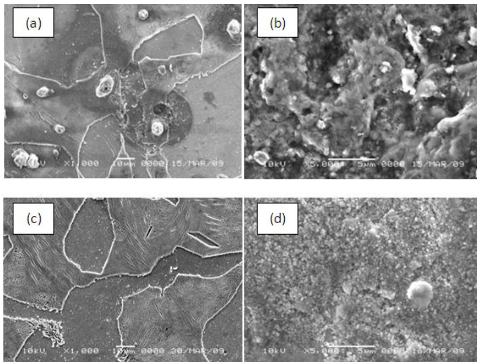
Figure 3: SEM micrographs high magnification of as cast Fe-Al-C alloy after corrosion (a). Fe-1.24Al-0.55C in 0.05 M H_2SO_4 (b). Fe-1.24Al-0.55C in NaCl c. Fe-9.05Al-0.6C in 0.05 M H_2SO_4 d. Fe-9.05Al-0.6C in NaCl
