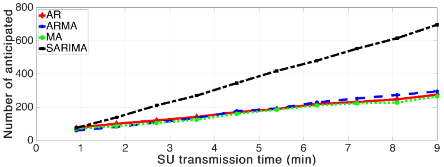
Fig. 3. Number of anticipated handoffs
